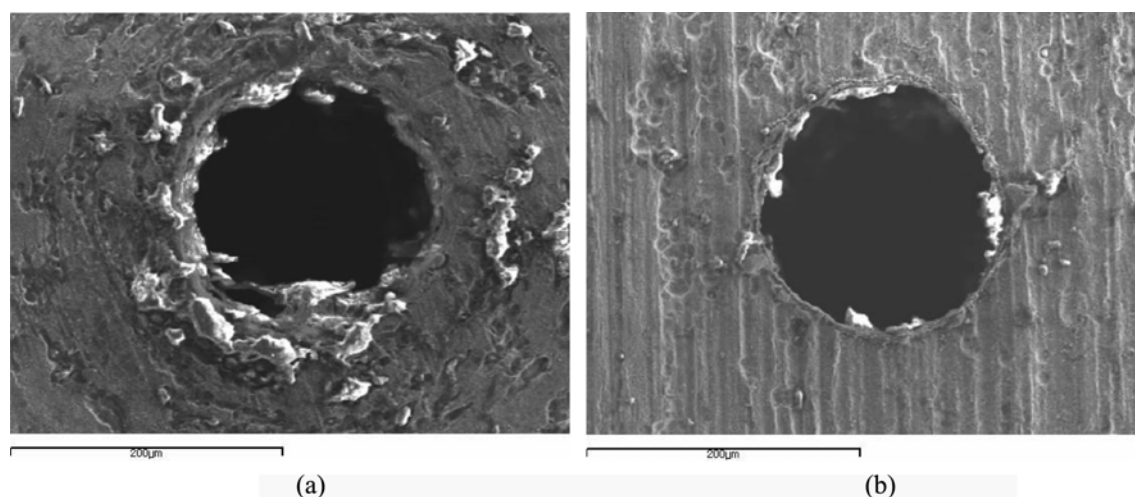
Fig. 3. SEM images of the nozzle surface after the sodium-water reaction. (a) 2.25Cr-1Mo (b) Mod.9Cr-1Mo
